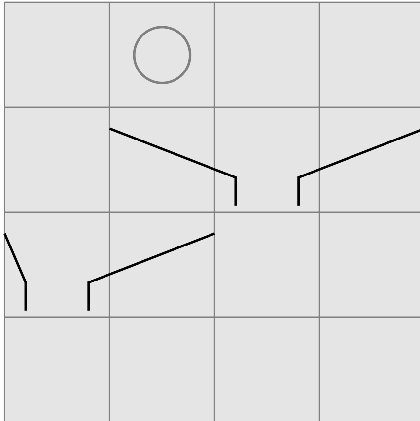
Figure: An example of the board of Pinball. M = 1 , N = 4 . A ball appears in the square (1, 2) in the first row. Then, the ball will move to (2, 2) , and it will be transferred to (2, 3) by the device 1. It finally arrives at the square (4, 3) in the bottom.
